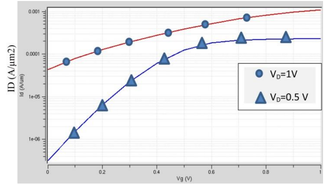
Fig. 3: Simulated I-V Characteristics for double gate FinFET for 40nm channel length
