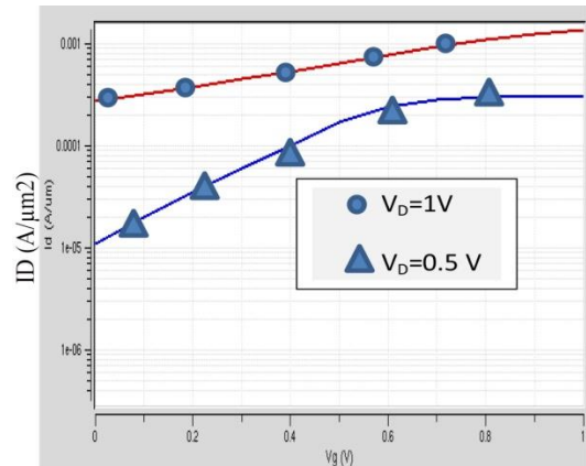
Fig. 5: Simulated I-V Characteristics for 60 nm Channel Length
