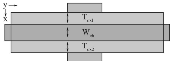
Fig. 2: Structure of FinFET showing oxide layers
