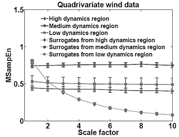
(a) Multivariate MSE
