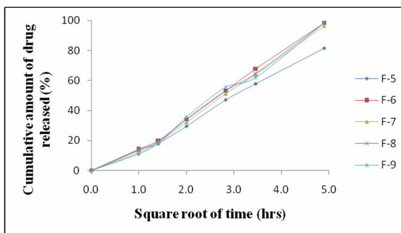
Figure 6. Higuchi's release profile of carvedilol for formulations F5 to F9 (mean; n=6).
