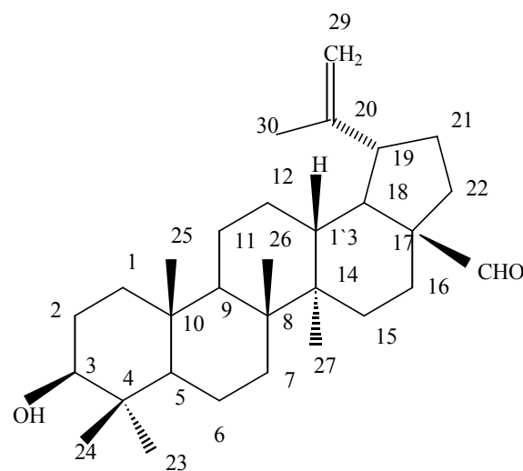
Betulinaldehyde as AO-3
