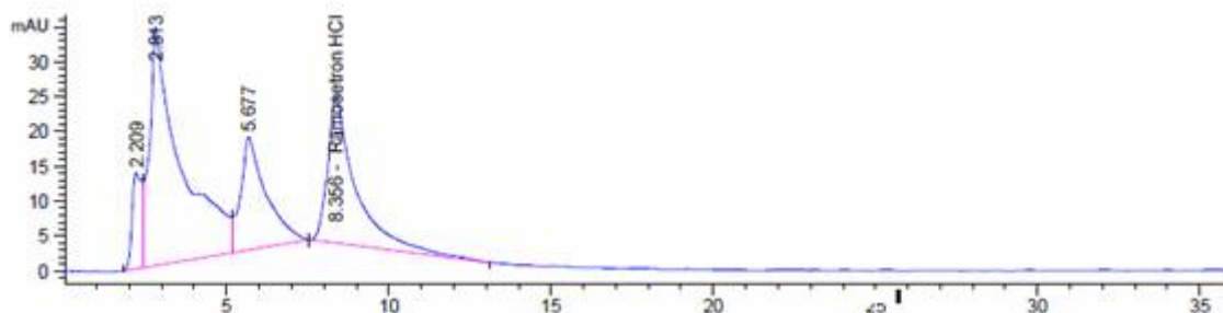
Figure 2. Chromatogram of Ramosetron HCl under stressed conditions with 0.1N NaOH for 2 days.
