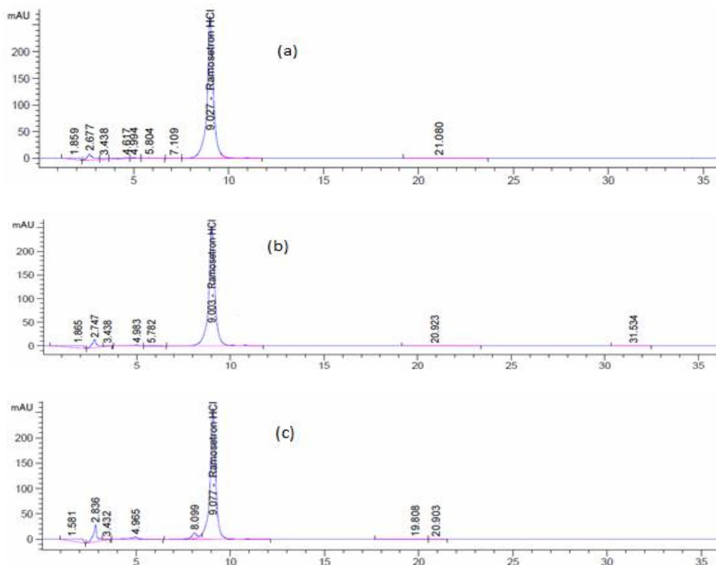
Figure 1. Chromatograms of Ramosetron HCl after 7 days stressed conditions (a) 0.5N HCl, (b) 1.0N HCl, (c) 2.0N HCl.
