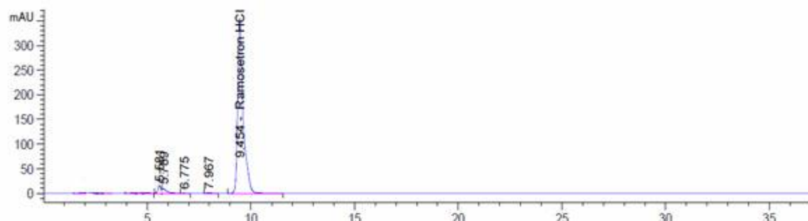
Figure 4. Chromatogram of Ramosetron HCl (Stressed sample exposed to 3.6 million lux fluorescence light and 600 watts hour/m 2 UV light).
