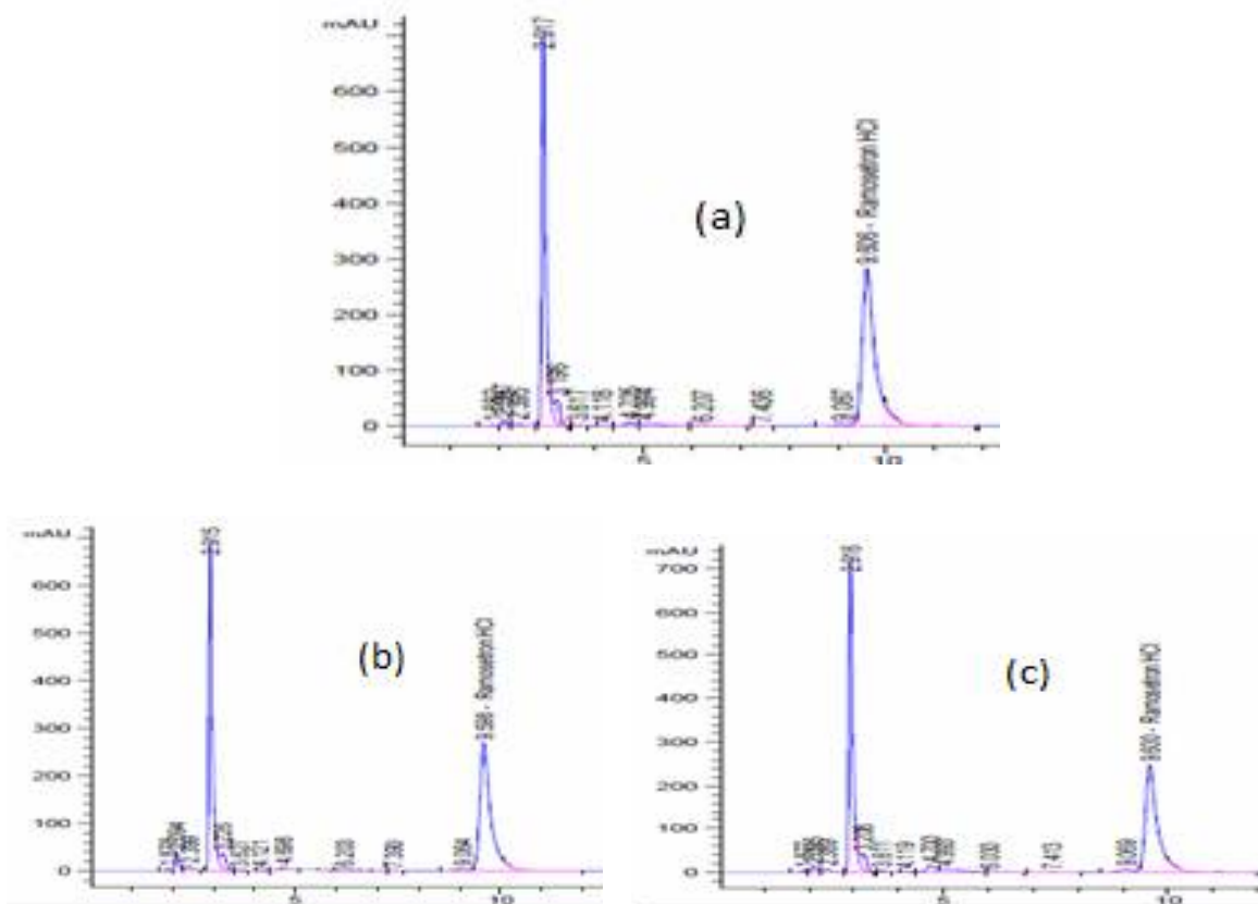
Figure 3. Chromatograms of stressed sample of Ramosetron HCl with 3% H 2 O 2 for (a) 1 hour, (b) 2 hours, (c) 3 hours.
