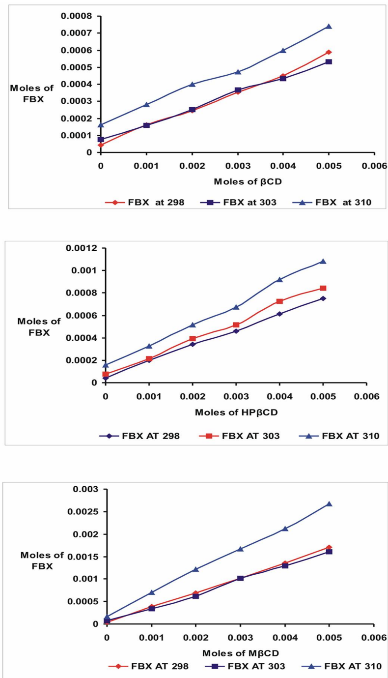
Figure 2. Phase solubility diagram of FBX: \beta CD, FBX:HP \beta CD, FBX:M \beta CD inclusion complexes at 298, 303, 310 \pm 2 K in acetate buffer pH 4.5. FBX: Febuxostat; \beta CD: \beta -cyclodextrin; HP \beta CD: Hydroxy propyl \beta -cyclodextrin; M \beta CD: Methyl \beta -cyclodextrin.
