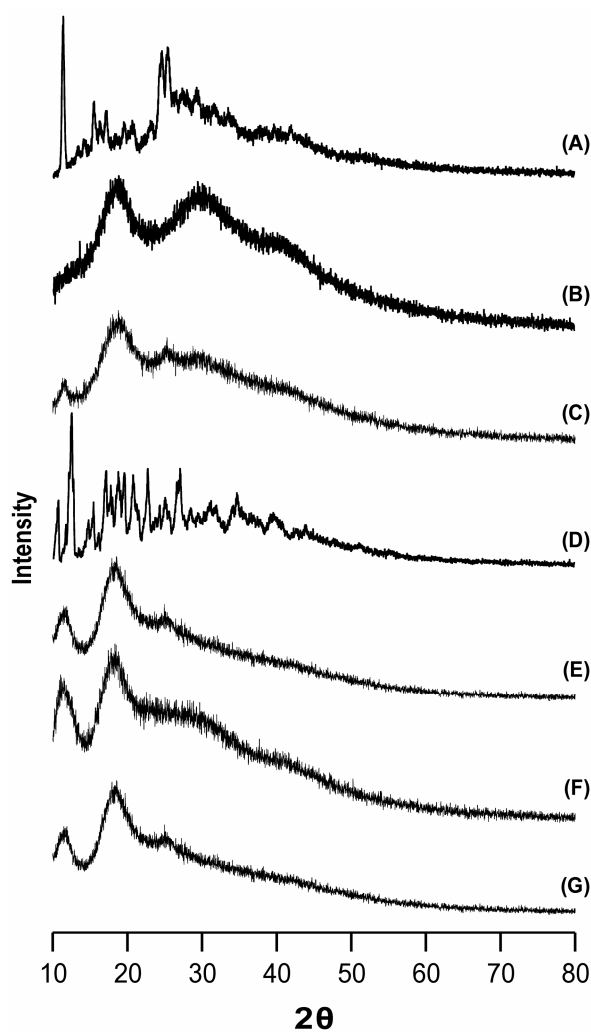
Figure 4. XRPD patterns of FBX (A), HPβCD (B), HPβCD complex (C), βCD (D), βCD complex (E), MβCD (F), MβCD complex (G). FBX: Febuxostat; βCD: β-cyclodextrin; HPβCD: Hydroxy propyl β-cyclodextrin; MβCD: Methyl β-cyclodextrin.
