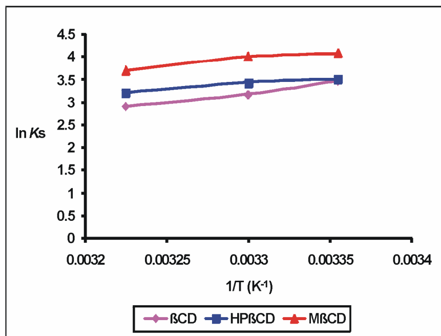
Figure 3. Van't Hoff plots ( \ln K vs 1/T ) for FBX: \beta CD, FBX:HP \beta CD, FBX:M \beta CD inclusion complexes, determined by solubility diagrams experiments. FBX:Febuxostat; \beta CD: \beta -cyclodextrin; HP \beta CD: Hydroxy propyl \beta -cyclodextrin; M \beta CD:Methyl \beta -cyclodextrin.
