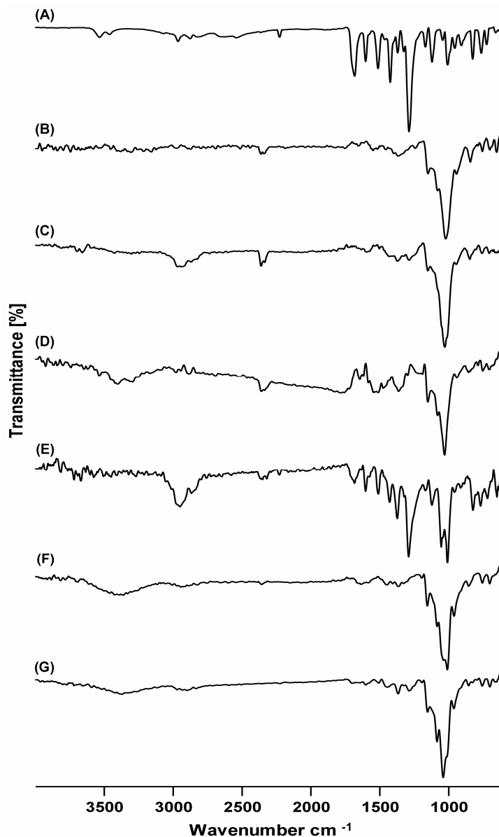
Figure 6. IR spectra FBX (A), HPβCD (B), HPβCD complex (C), βCD (D), βCD complex (E), MβCD (F), MβCD complex (G). FBX: Febuxostat; βCD: β-cyclodextrin; HPβCD: Hydroxy propyl β-cyclodextrin; MβCD: Methyl β-cyclodextrin.
