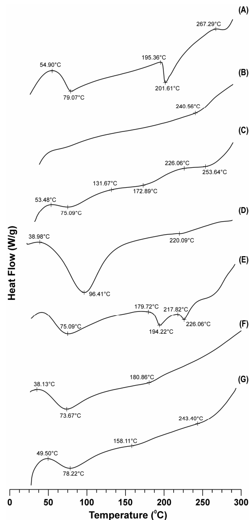
Figure 5. DSC thermograms of FBX (A), HPβCD (B), HPβCD complex (C), βCD (D), βCD complex (E), MβCD (F), MβCD complex (G). FBX: Febuxostat; βCD: β-cyclodextrin; HPβCD: Hydroxy propyl β-cyclodextrin; MβCD: Methyl β-cyclodextrin.
