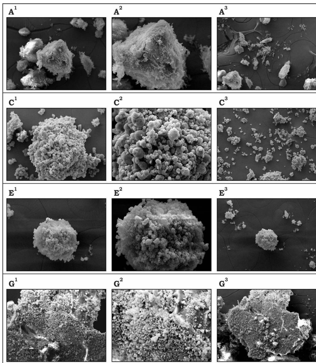
Figure 7. SEM of FBX (A), HP \beta CD complex (C), \beta CD complex (E), M \beta CD complex (G) 1 1kx magnification; 2 2kx magnification; 3 500x magnification. FBX: Febuxostat; \beta CD: \beta -cyclodextrin; HP \beta CD: Hydroxy propyl \beta -cyclodextrin; M \beta CD: Methyl \beta -cyclodextrin.
