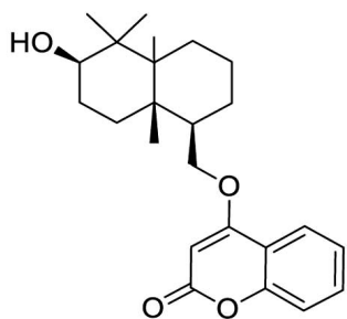
Foetidin (6)
