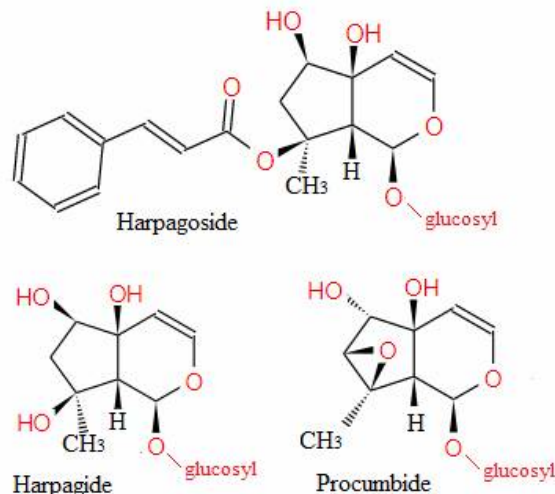
Figure 1. Iridoid glycosides of devil's claw
