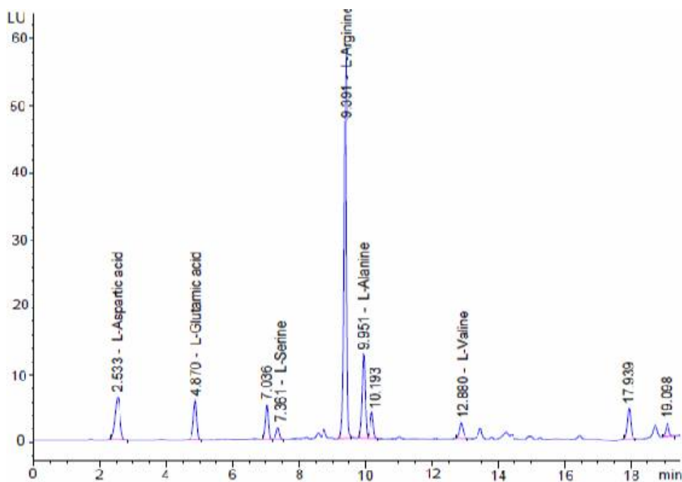
Figure 3. Chromatogram (HPLC) of the free amino acids in the roots of Harpagophytum procumbens .
