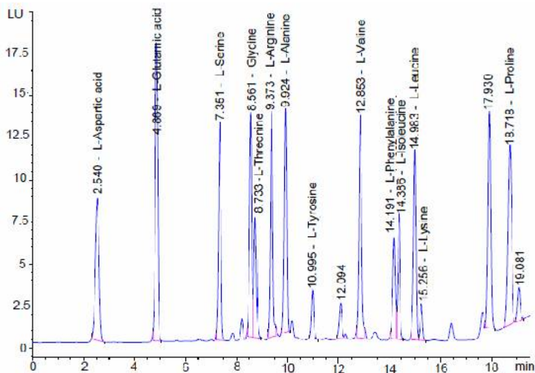
Fig. 4. Chromatogram (HPLC) of the total amino acids in the roots of Harpagophytum procumbens .
