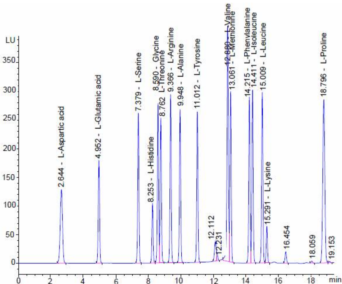
Figure 2. Chromatogram of the standard amino acid mixture.
