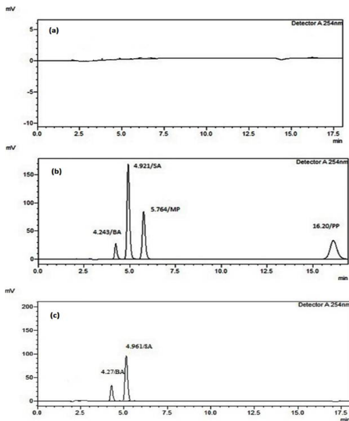
Figure 2. Chromatograms of blank (a), standard solution (b) and a sample (c).
