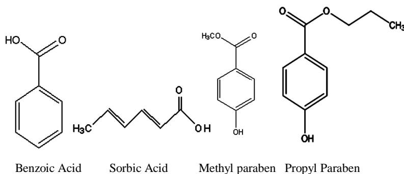
Figure 1. Chemical Structure of BA, SA, MP and PP.
