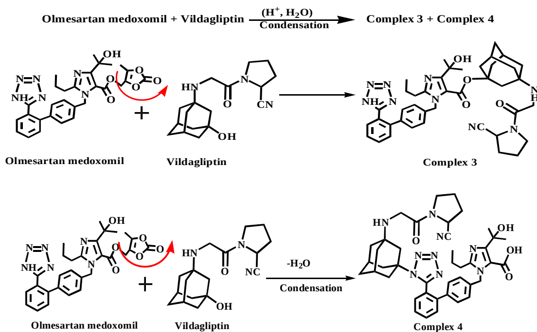
Figure 10. Postulated complexation patterns between olmesartan medoxomil and vildagliptin.
