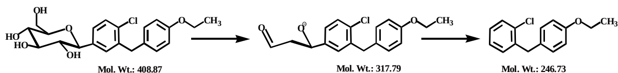
Figure 5. Degradation pattern of dapagliflozine.
