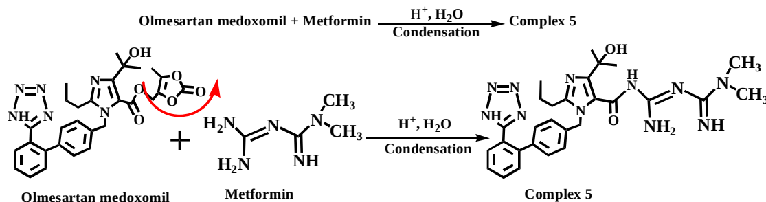
Figure 11. Postulated complexation patterns between olmesartan medoxomil and metformin.
