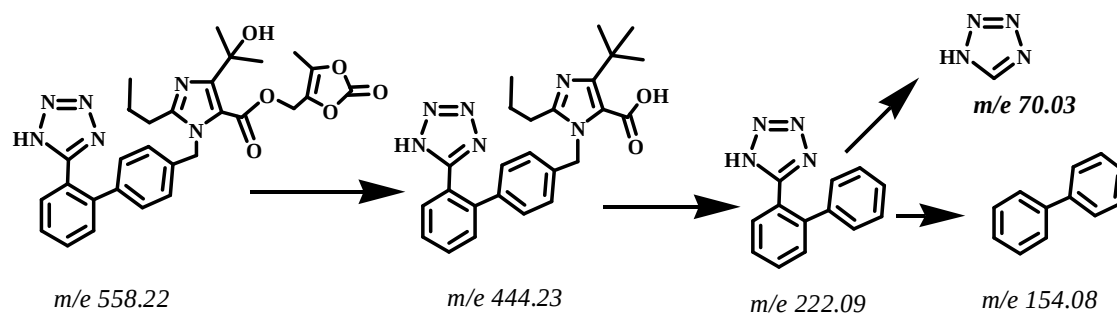
Figure 4. Degradation pattern of olmesartan medoxomil.
