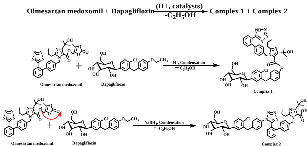
Figure 9. Postulated complexation patterns between olmesartan medoxomil and dapagliflozin.
