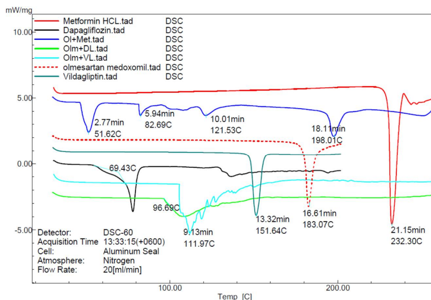
Figure 2. Overlaid DSC thermograms of olmesartan medoxomil, dapagliflozin, vildagliptin, metformin and their complexes.
