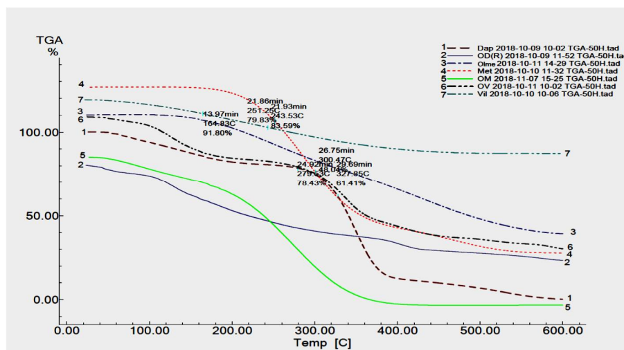
Figure 3. Overlaid TGA of pure drugs and their complexes.
