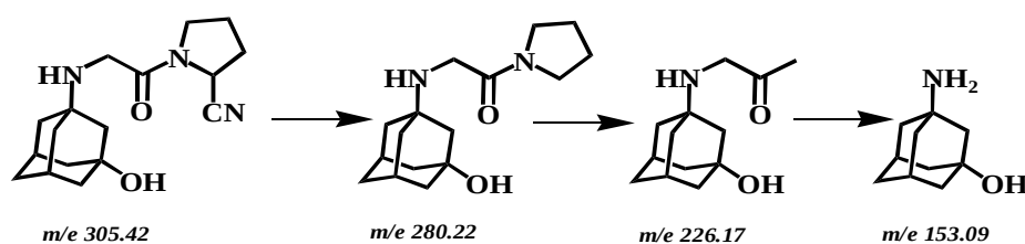
Figure 6. Degradation pattern of vildagliptin.
