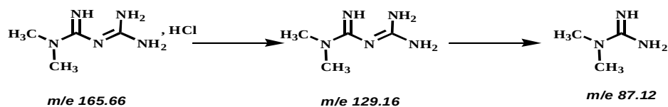
Figure 7. Degradation pattern of metformin HCl.
