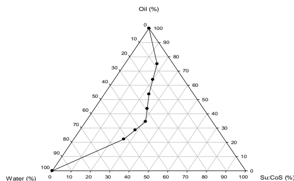
Figure 1. Pseudo ternary phase diagram of 1:1 Su:CoSu.
