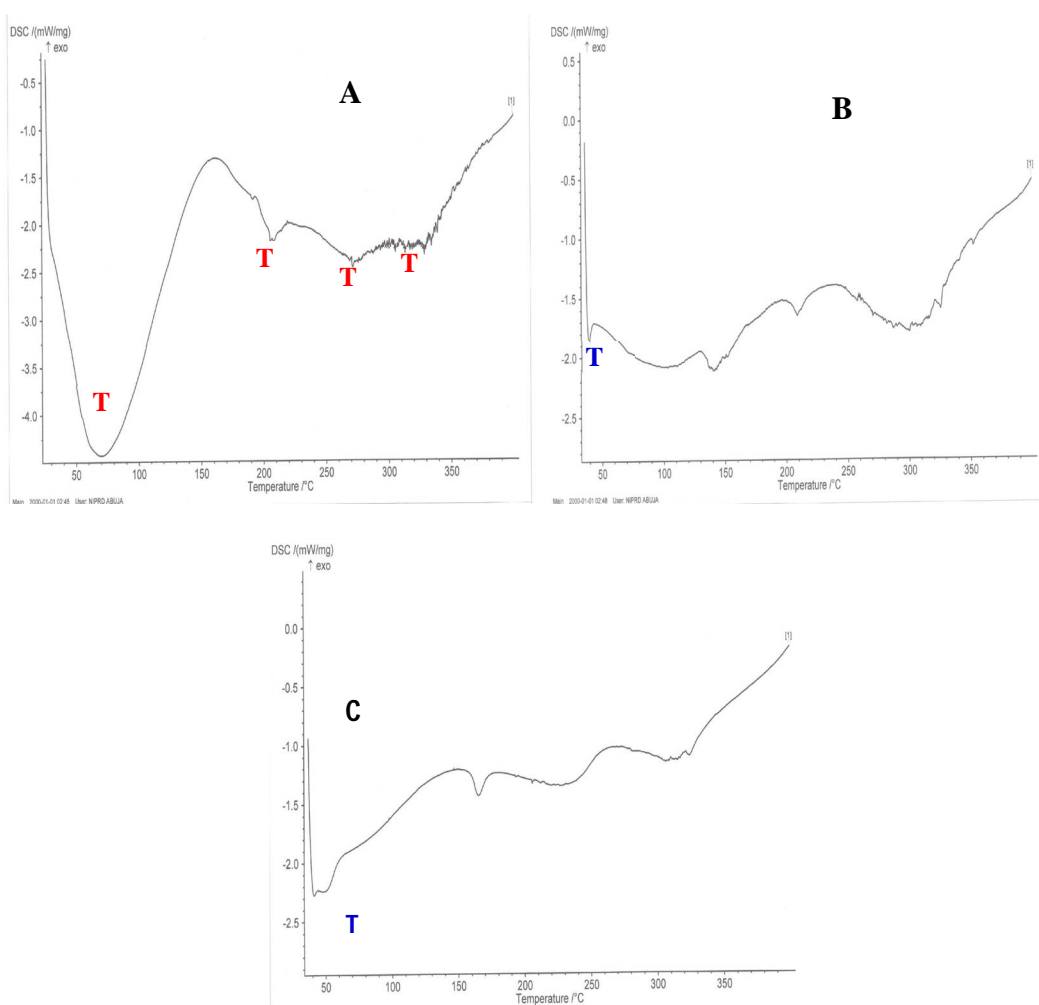
Figure 3. DSC thermograms of: (A) untreated (B) M2- and (C) 9:1 ethanol co-solvent-treated SC.
