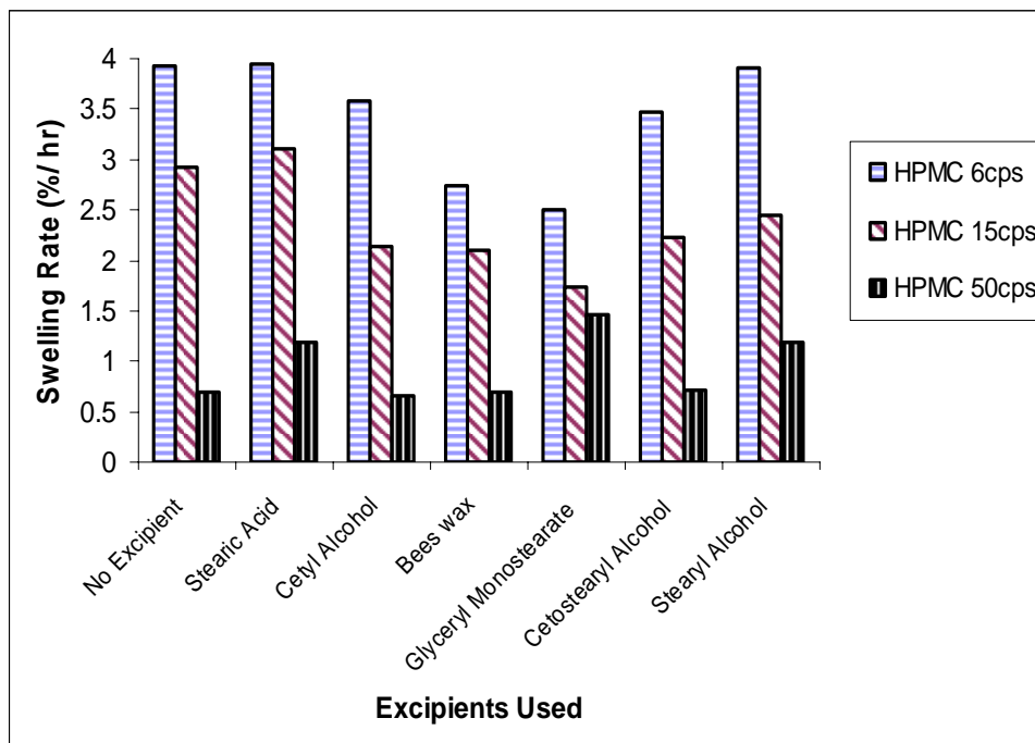
Figure 6. Effect on swelling rates of different excipients with different grades of HPMC.
