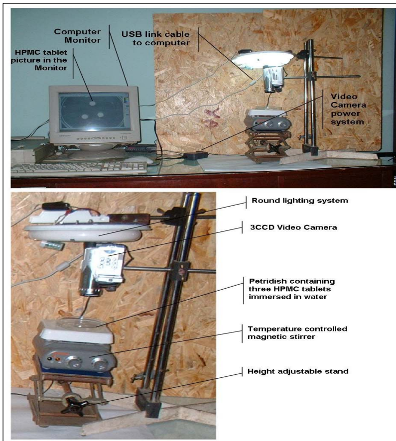
Figure 1. The video camera and computer setup along with the sampling petridish for snap shots of swelling of HPMC tablets.
