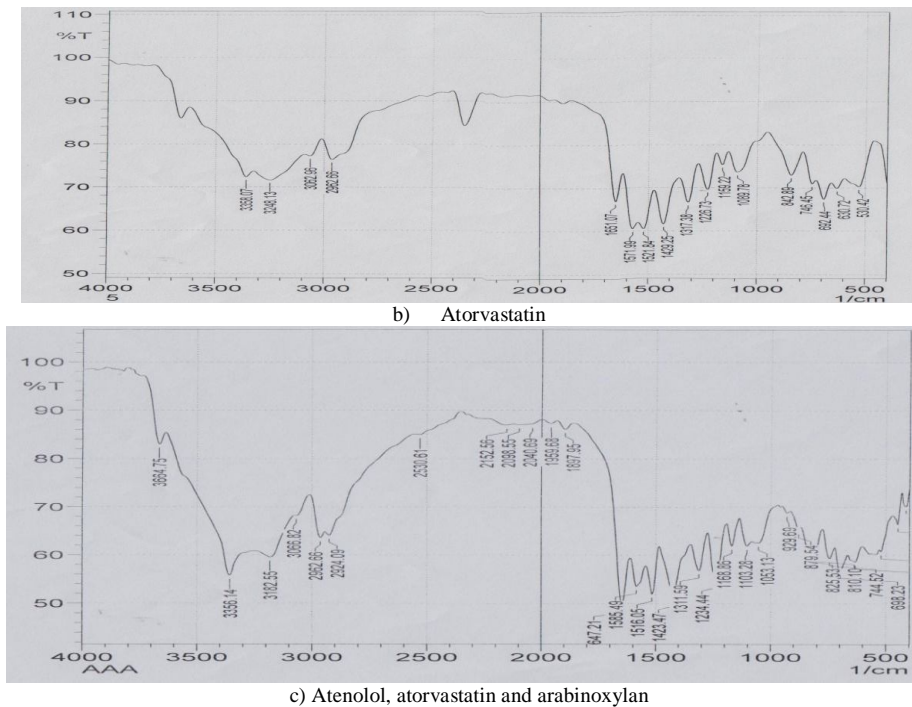
Figure 1. FTIR spectra of atenolol, atorvastatin and physical blend of drugs with arabinoside.
