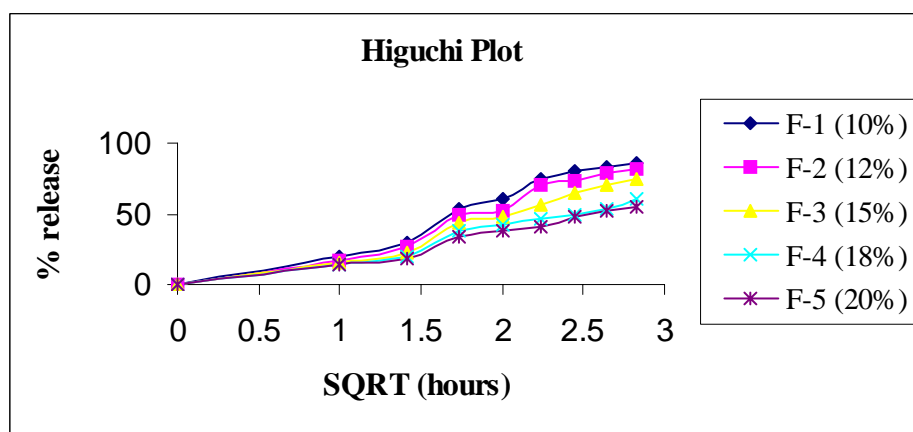
Figure 2. Effect of kollidon SR on theophylline from proposed formulations in gastrointestinal fluid and intestinal fluid (Higuchi plot).
