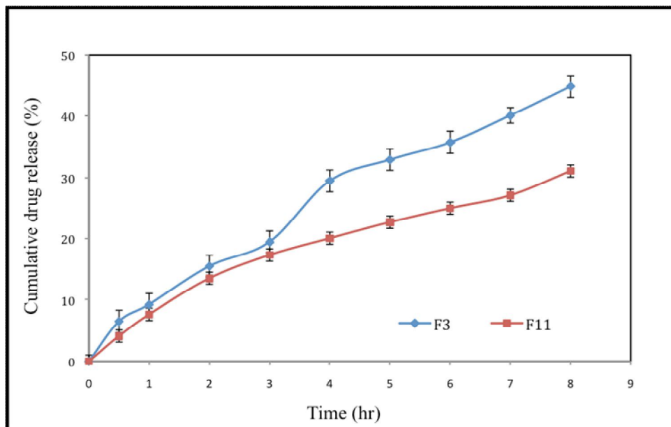
Figure 3. Effect of polymer concentration and viscosity (HPMC K4M and Carbopol 971) on drug release rate.
