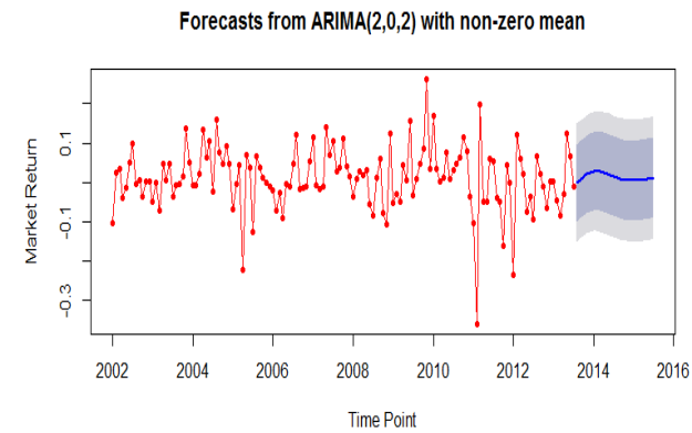
Fig. 4. Performance of ARIMA (2, 0, 2) model
