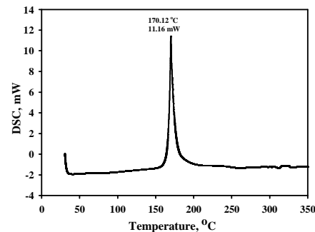
Fig. 5. DSC graph of [\text{Hg}(\text{RPZ})_2] \cdot \text{H}_2\text{O} .
