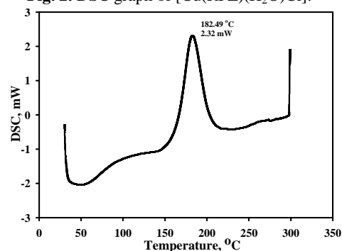
Fig. 3. DSC graph of [\text{Zn}(\text{RPZ})_2] .
