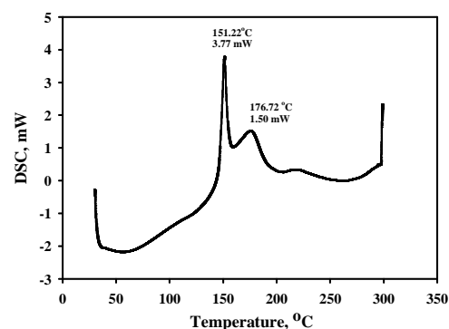
Fig. 2. DSC graph of [\text{Cu}(\text{RPZ})(\text{H}_2\text{O})\text{Cl}] .
