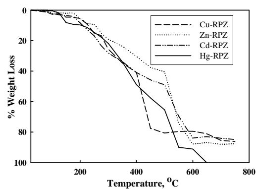
Fig. 1. QSTG graphs of Cu(II), Zn(II), Cd(II) and Hg(II) complexes of rabeprazole.
