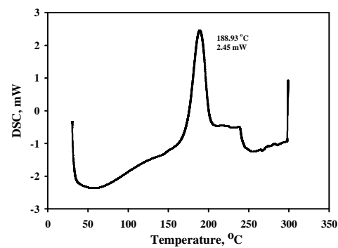
Fig. 4. DSC graph of [\text{Cd}(\text{RPZ})_2] \cdot 2\text{H}_2\text{O} .
