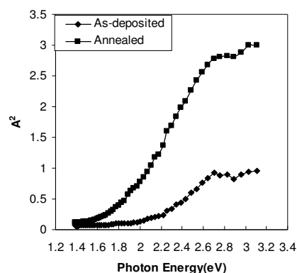
Fig. 1. Estimation of band gap ( E_g ) of as-deposited and annealed CdSe thin film.
