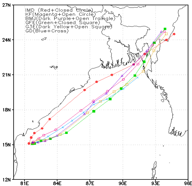
Fig. 1. The IMD observed and WRF model simulated 72 hours track forecast of TC Roanu for five different CP schemes starting from 0000 UTC of 19 May to 0000 UTC of 22 May 2016.
