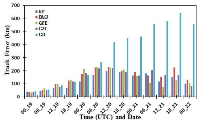
Fig. 2. The variation of track error with time for five different CP schemes.
