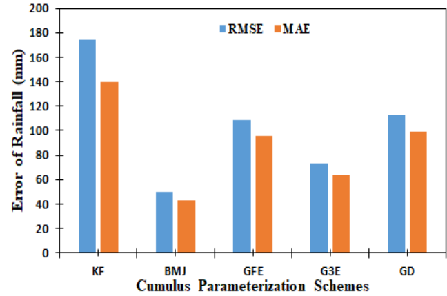
Fig. 9. The RMSE and MAE of rainfall for five different CP schemes.
