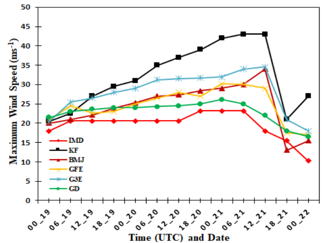
Fig. 5. Variation of observed and model simulated MWS (ms -1 ) with time for five different CP schemes.
