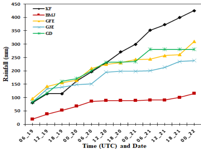
Fig. 8. The time variation of model simulated accumulated rainfall (mm) for five different CP schemes.
