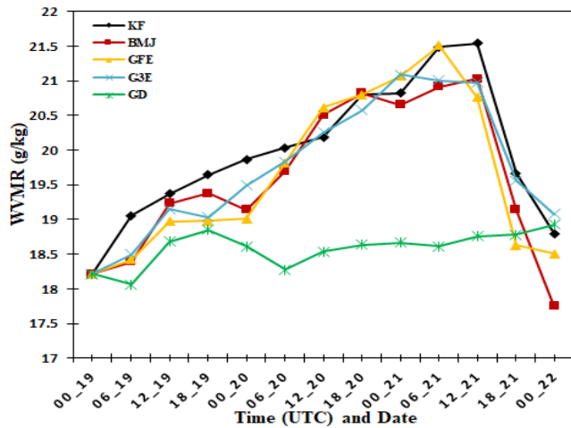
Fig. 10. Variation of model simulated area average WVMR (g/kg) at 850 hPa level with time for five different CP schemes.
