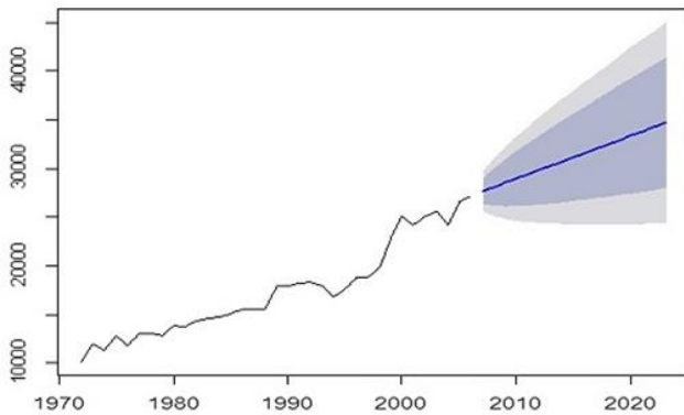
Fig. 3. Forecasts for ARIMA (1,1,1).
