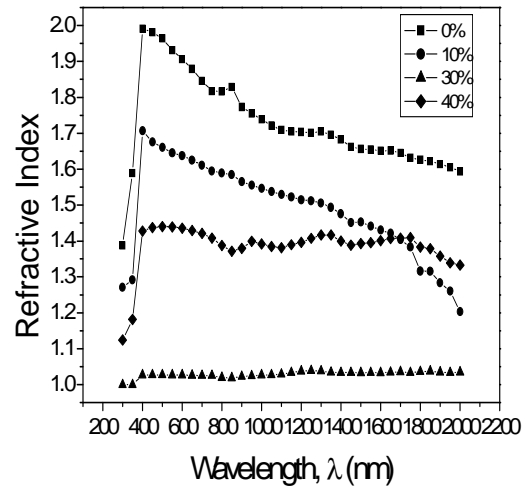
Fig. 5. Variation of refractive index with wavelength for pure and Mg-doped ZnO thin films
