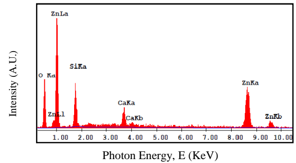
Fig. 6. EDX spectra of Pure ZnO thin film
