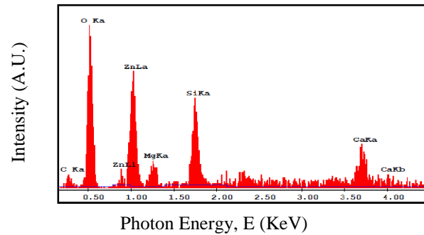
Fig. 7. EDX Spectra of as deposited 10% Mg doped ZnO thin film
