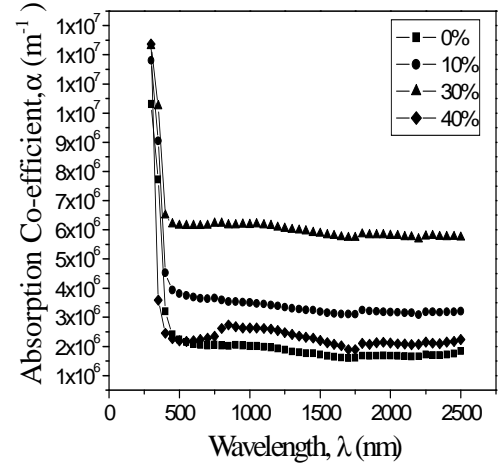
Fig. 2. Variation of absorption co-efficient with wavelength for pure and Mg-doped ZnO thin films
