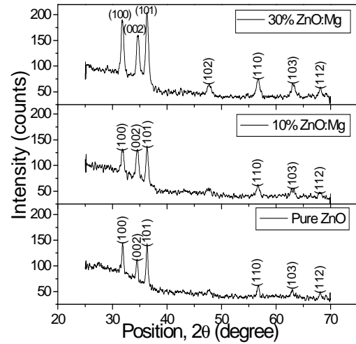
Fig. 10. XRD pattern of pure ZnO, 10% and 30% Mg doped ZnO thin film annealed at 425^\circ\text{C}
