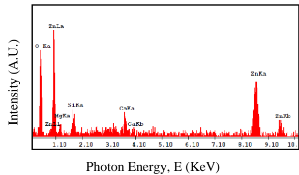
Fig. 8. EDX Spectra of as deposited 30% Mg doped ZnO thin film
