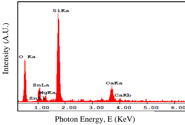
Fig. 9. EDX Spectra of as deposited 40% Mg doped ZnO thin film
