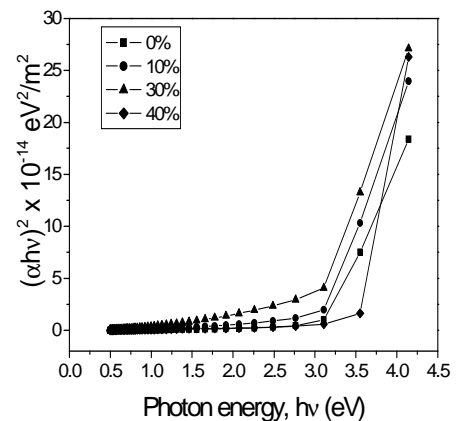
Fig. 3. (\alpha h\nu)^2 versus photon energy graph for pure and Mg-doped ZnO thin films
