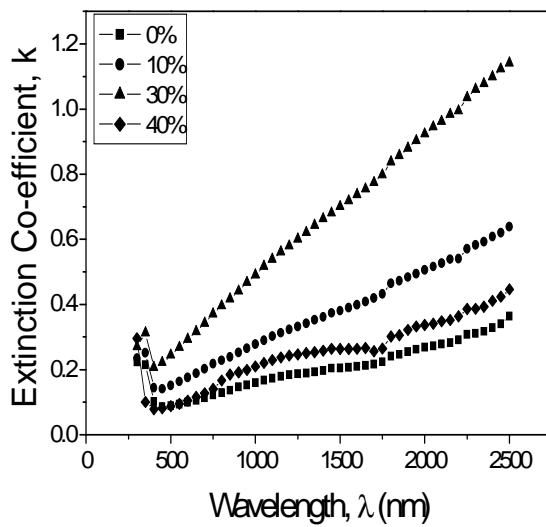
Fig.4. Variation of extinction co-efficient with wavelength for pure and Mg-doped ZnO thin films
