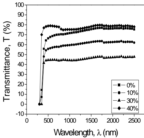
Fig.1. Transmittance versus wavelength graph for pure and Mg-doped ZnO thin films
