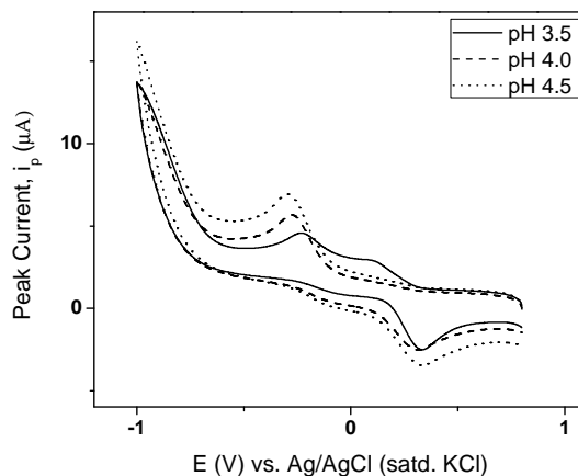
Fig. 3. CVs of 1.0 mM Fe(III) in acetate buffer solution at pH (a) 3.5 (solid), (b) 4.0 (dot-dashed) and (c) 4.5 (dotted).
