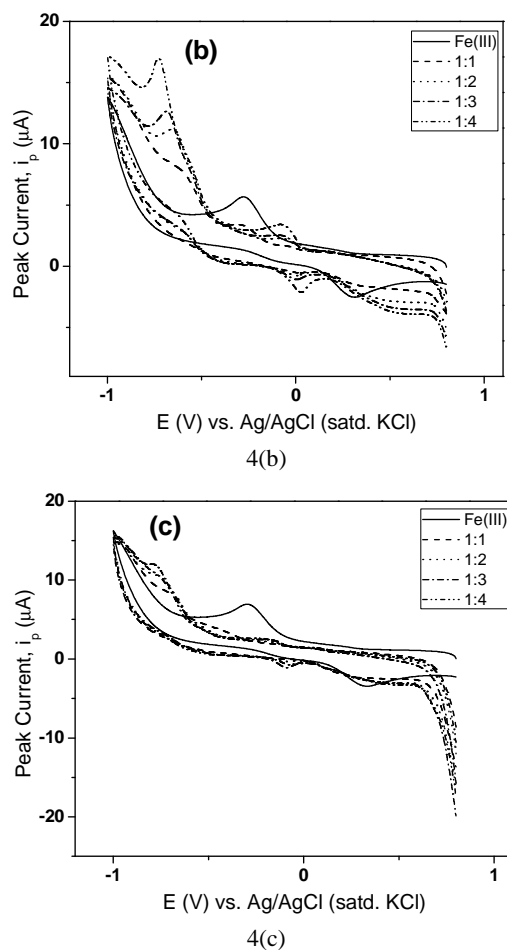
Fig. 4. CVs of Fe(III) (solid), and Fe(III)/Ome with different ratio (i) 1:1 (dot-dashed), (c) 1:2 (dotted), (d) 1:3 (long-dashed), and (e) 1:4 (medium-dashed) in acetate buffer solution at (a) pH 3.5, (b) pH 4.0 and (c) pH 4.5.
