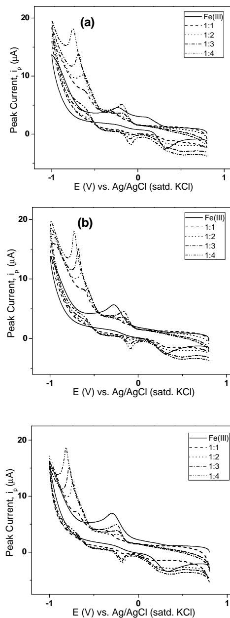
Fig. 7. CVs of Fe(III) (solid), and Fe(III)/Rab with different ratio (i) 1:1 (dot-dashed), (ii) 1:2 (dotted), (iii) 1:3 (long-dashed), and (iv) 1:4 (medium-dashed) in acetate buffer solution at (a) pH 3.5, (b) pH 4.0 and (c) pH 4.5.
