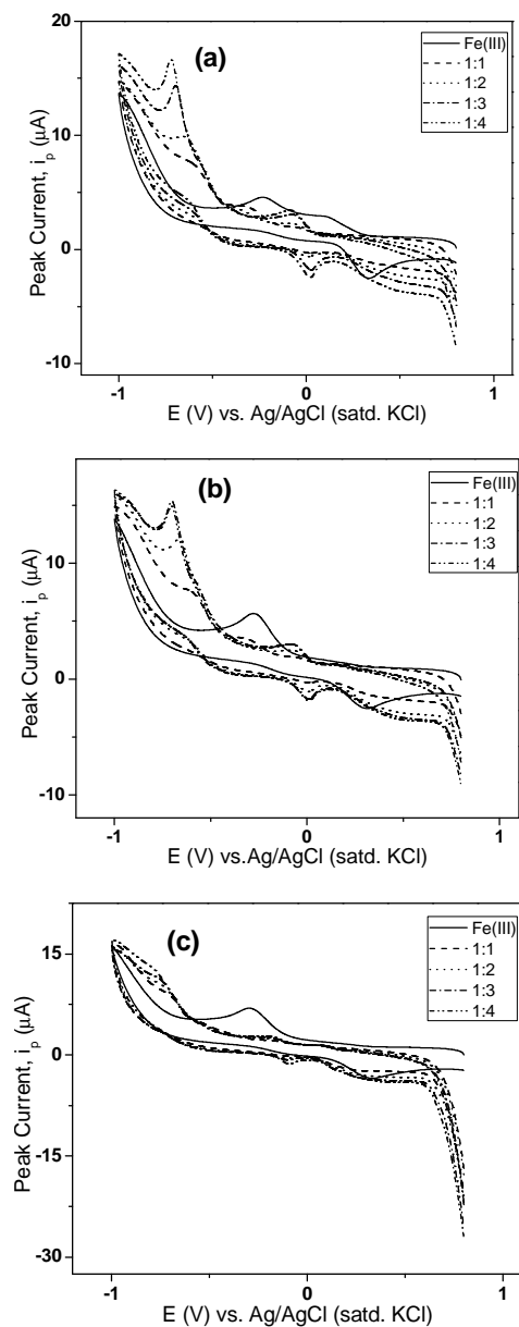
Fig. 6. CVs of Fe(III) (solid), and Fe(III)/Eso with different molar ratio (i) 1:1 (dot-dashed), (ii) 1:2 (dotted), (iii) 1:3 (long-dashed), and (iv) 1:4 (medium-dashed) in acetate buffer solution at (a) pH 3.5, (b) pH 4.0 and (c) pH 4.5.
