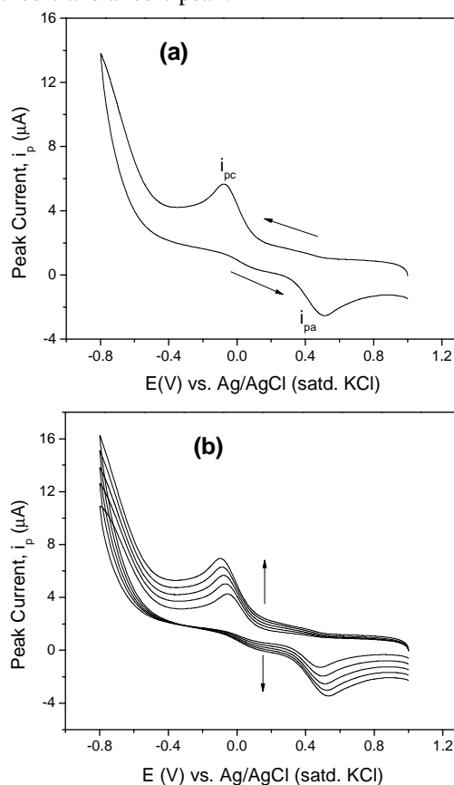
Fig. 1. CV of (a) 1.0 mM Fe(III) in acetate buffer solution at pH 4.0 with scan rate of 100 mVs -1 and (b) CVs of 1.0 mM Fe(III) at various scan rate: 50, 75, 100, 125 and 150 mVs -1 at GCE.
