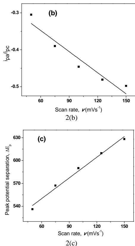
Fig. 2. (a) Plots of cathodic peak current (i) and anodic peak current (ii) as a function of square root of scan rate, (b) Peak current ratio ( i_{pa}/i_{pc} ) dependence on scan rate and (c) A plot of peak potential separation with scan rate for 1.0 mM Fe(III) at pH 4.0.
