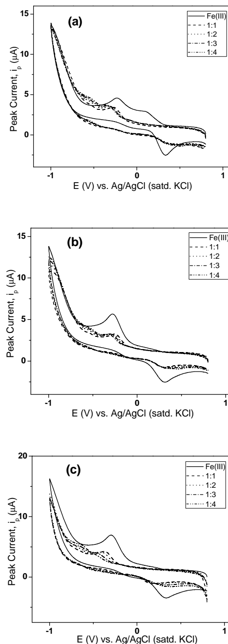
Fig. 5. CVs of Fe(III) (solid), and Fe(III)/Pan with different ratio (i) 1:1 (dot-dashed), (ii) 1:2 (dotted), (iii) 1:3 (long-dashed), and (iv) 1:4 (medium-dashed) in acetate buffer solution at (a) pH 3.5, (b) pH 4.0 and (c) pH 4.5.
