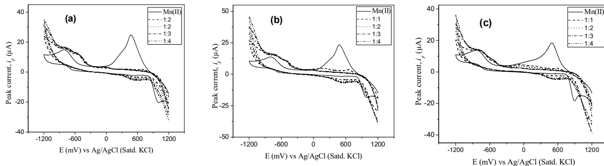
Fig. 6. CVs of Mn^{2+} (solid), and Mn^{2+}/Eso with different ratio (i) 1:1 (dash), (ii) 1:2 (dot), (iii) 1:3 (dash dot), and (iv) 1:4 (dash dot dot) in acetate buffer solution at (a) pH 3.5, (b) pH 4.0 and (c) pH 4.5.
