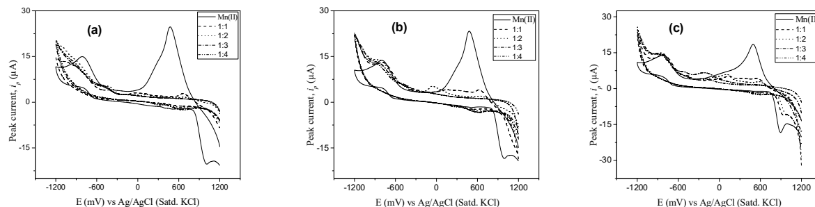
Fig. 5. CVs of Mn^{2+} (solid), and Mn^{2+}/Pan with different ratio (i) 1:1 (dash), (ii) 1:2 (dot), (iii) 1:3 (dash dot), and (iv) 1:4 (dash dot dot) in acetate buffer solution at (a) pH 3.5, (b) pH 4.0 and (c) pH 4.5.
