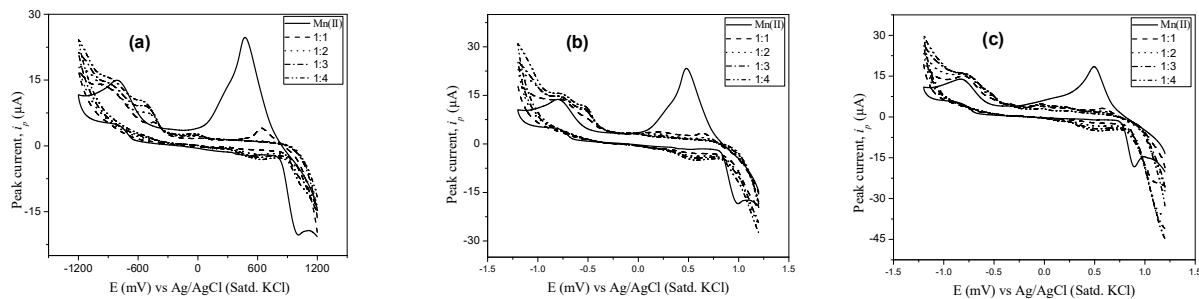
Fig. 4. CVs of Mn^{2+} (solid), and Mn^{2+}/Ome with different ratio (i) 1:1 (dash), (ii) 1:2 (dot), (iii) 1:3 (dash dot), and (iv) 1:4 (dash dot dot) in acetate buffer solution at (a) pH 3.5, (b) pH 4.0 and (c) pH 4.5.
