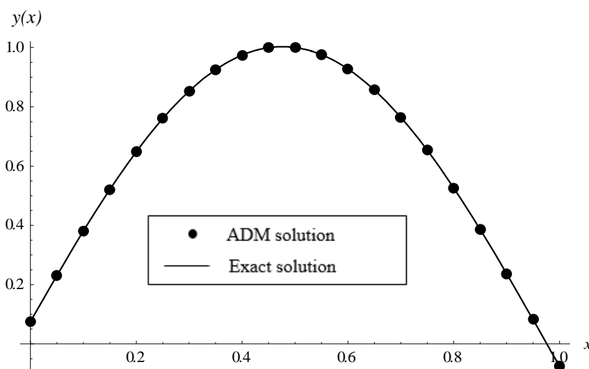
Fig. 2. Solutions to the integral equation (5)
