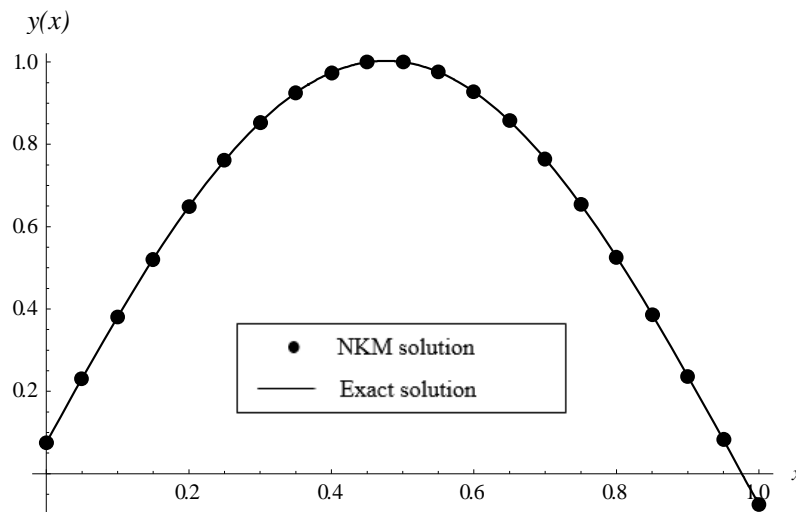
Fig. 1. Solutions to the integral equation (5)
